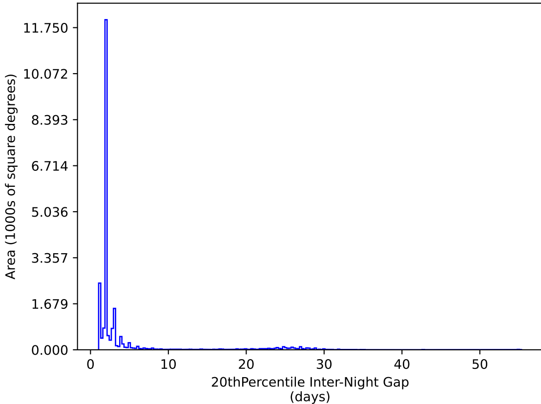
too_ignore_10_1v3.4_10yrs All sky y band: 20thPercentile Inter-Night Gap
