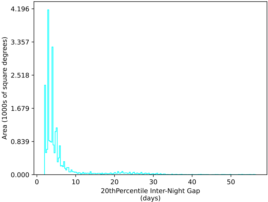
too_ignore_10_1v3.4_10yrs All sky u band: 20thPercentile Inter-Night Gap
