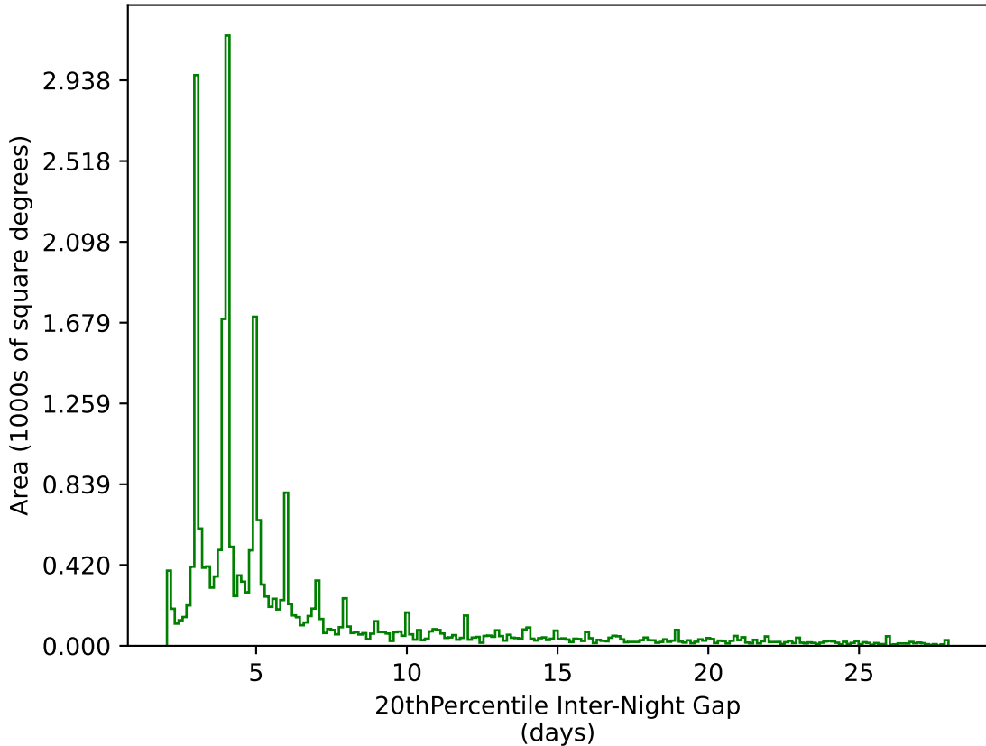
too_ignore_10_1v3.4_10yrs All sky g band: 20thPercentile Inter-Night Gap
