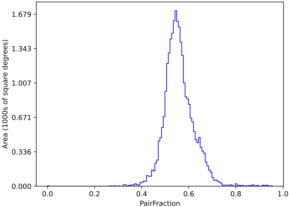
too_ignore_10_1v3.4_10yrs (g or r or i): PairFraction
