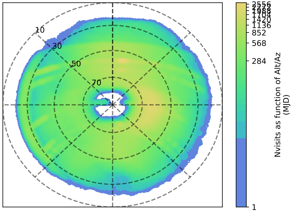
too_ignore_10_1v3.4_10yrs r: Nvisits as function of Alt/Az
