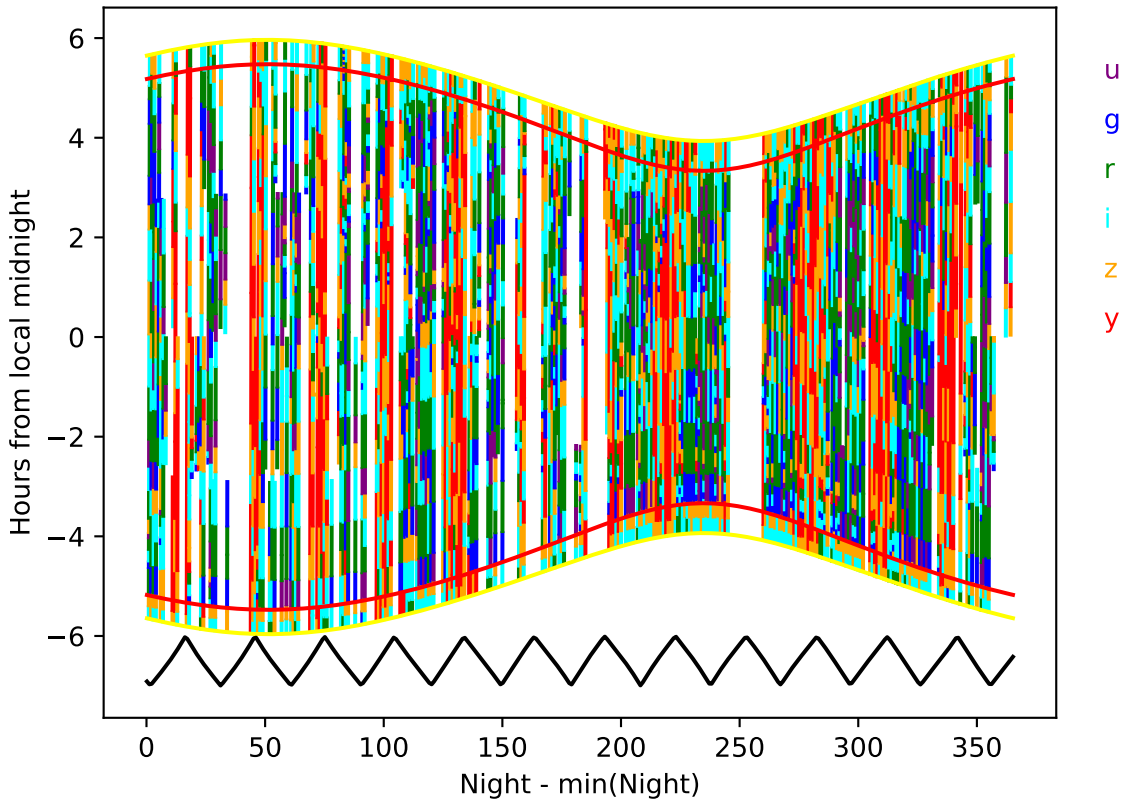
too_ignore_10_1v3.4_10yrs year 5-6: Hourglass
