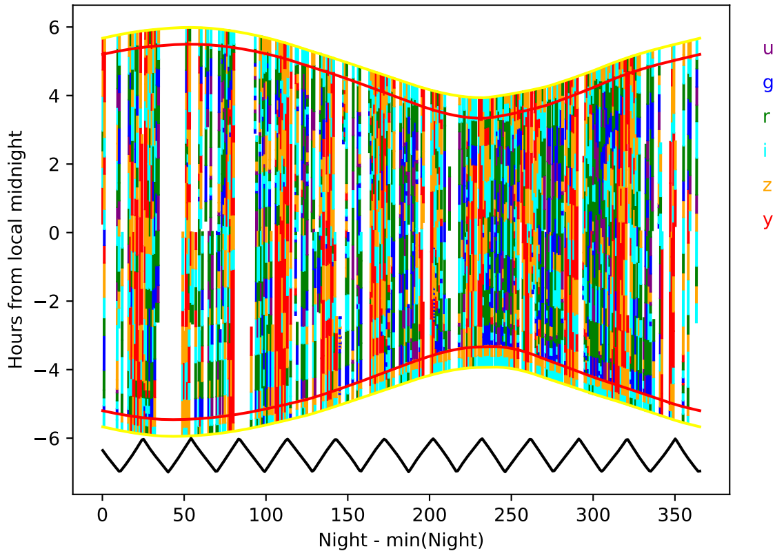
too_ignore_10_1v3.4_10yrs year 4-5: Hourglass
