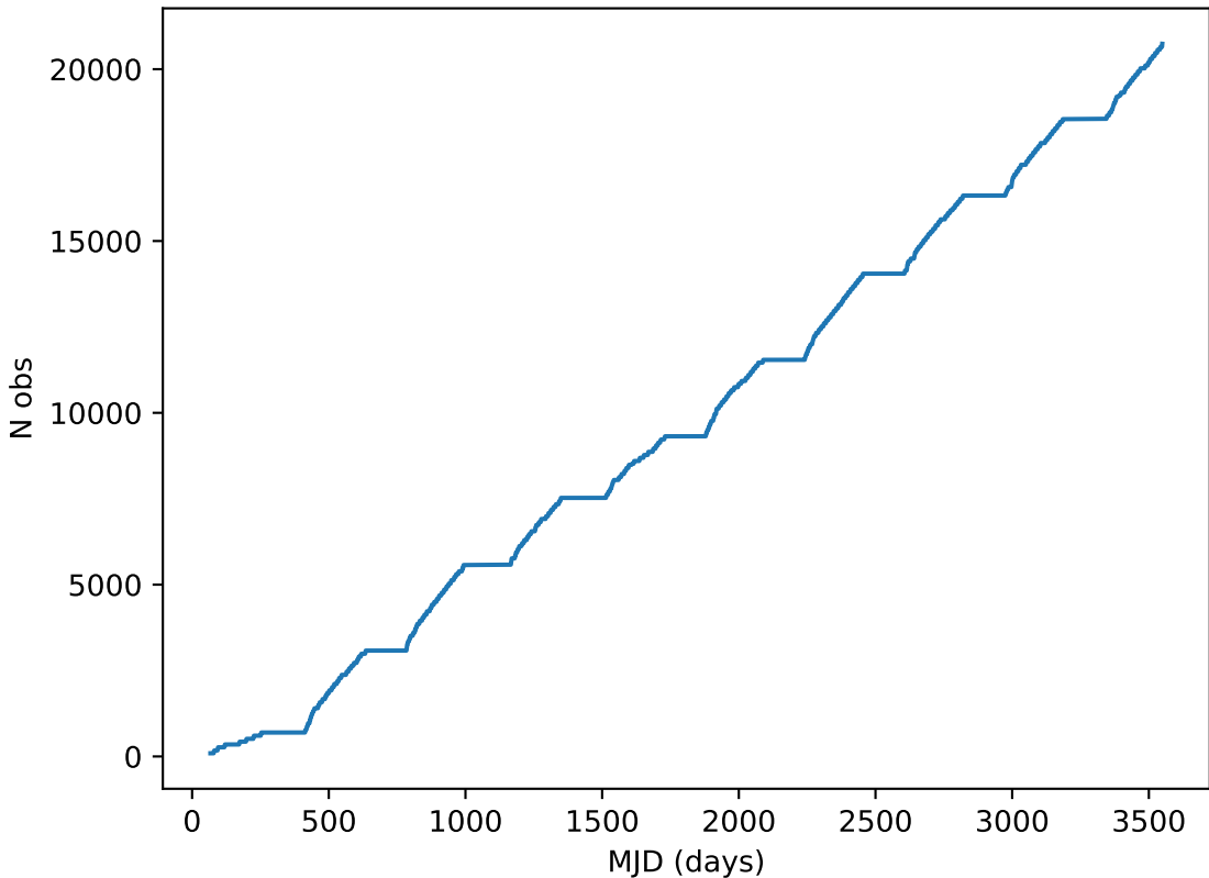
too_ignore_10_1v3.4_10yrs note like DD:ELAISS1%: Cumulative
