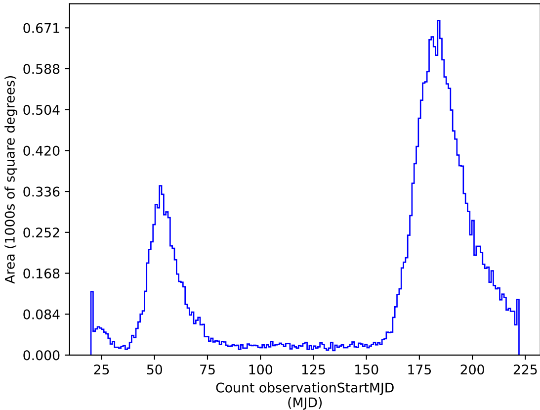
too_ignore_10_1v3.4_10yrs r: Count observationStartMJD
