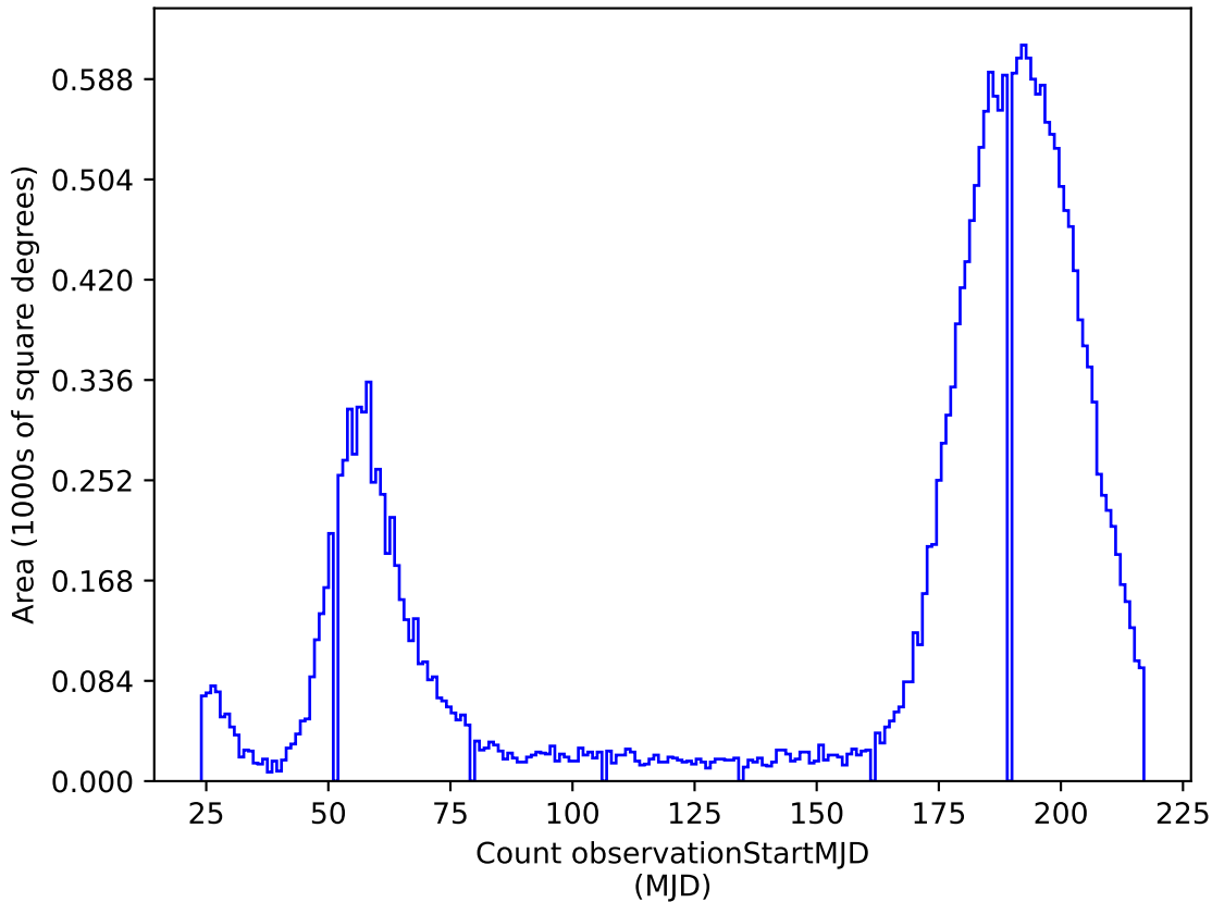
too_ignore_10_1v3.4_10yrs i: Count observationStartMJD
