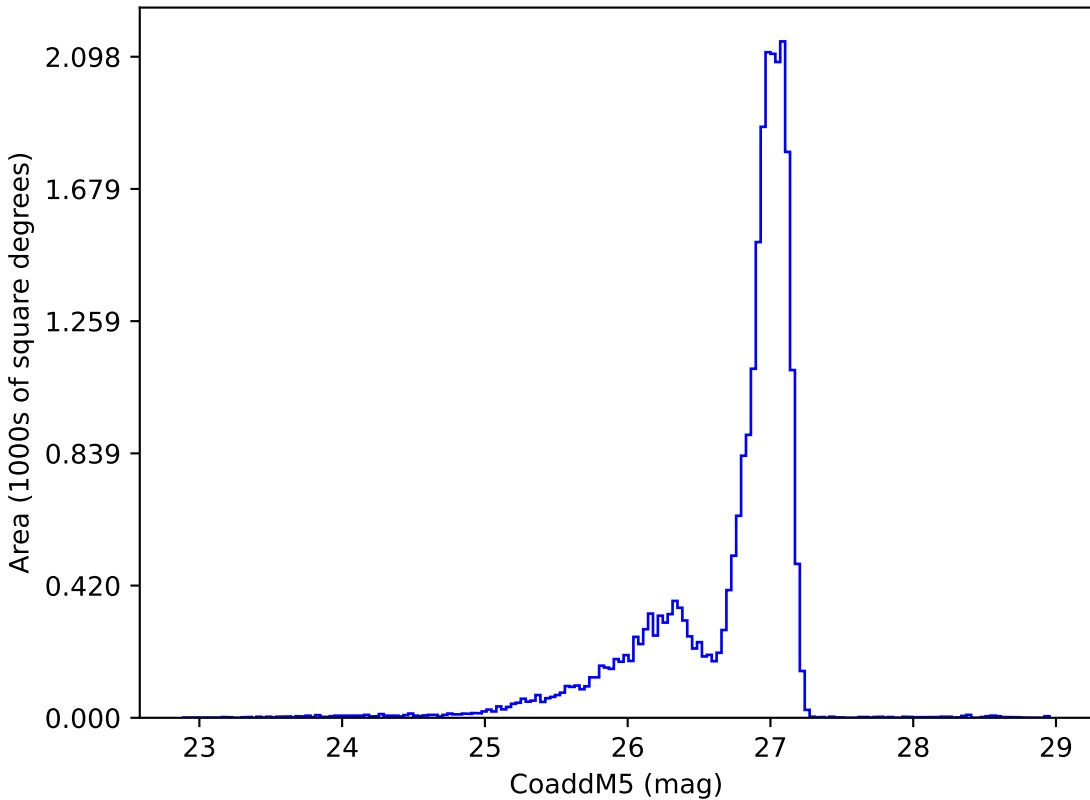
too_ignore_10_1v3.4_10yrs r: CoaddM5
