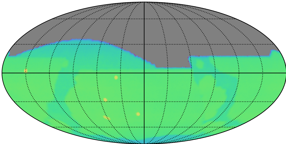
too_ignore_10_1v3.4_10yrs : CoaddM5
