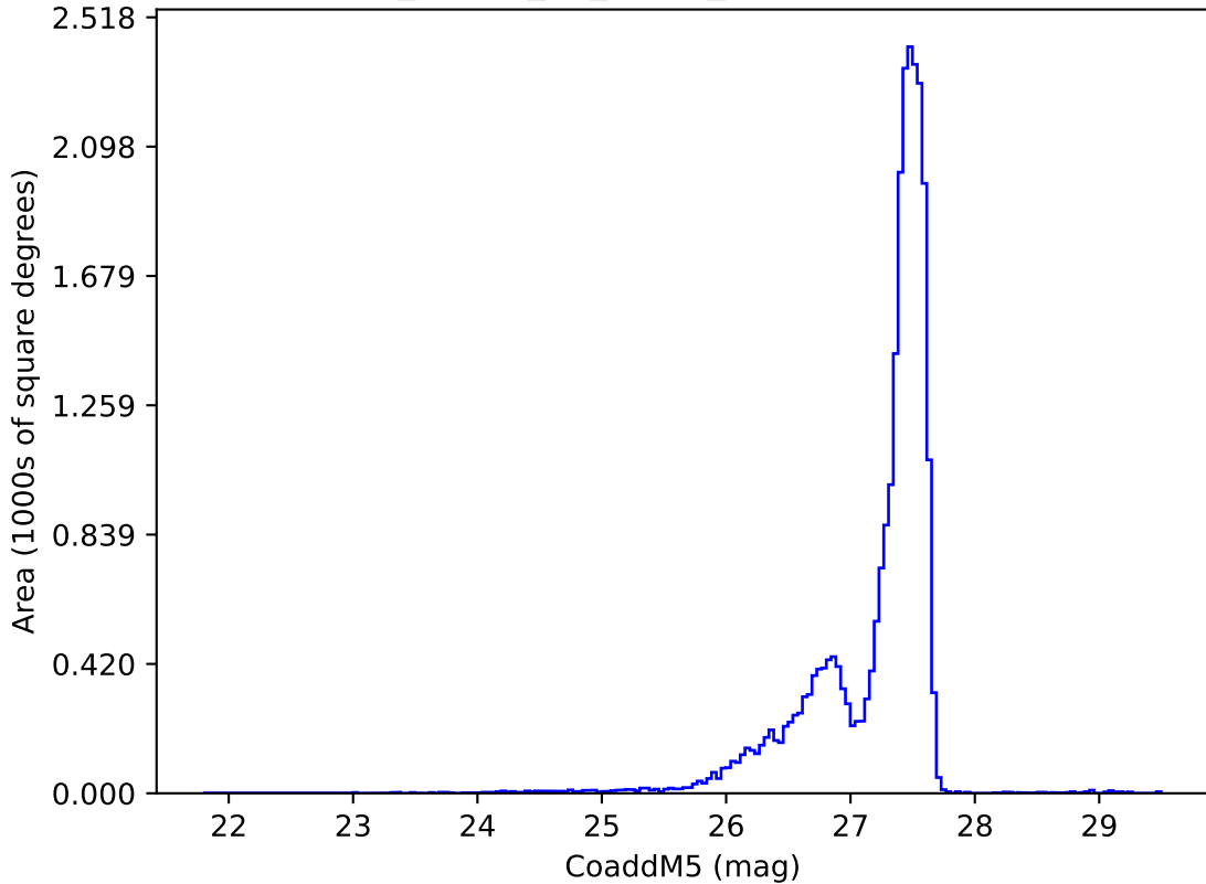
too_ignore_10_1v3.4_10yrs : CoaddM5
