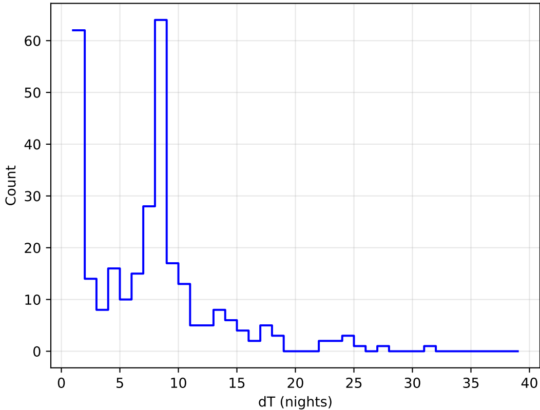
too_ignore_10_1v3.4_10yrs all bands: DD:XMM_LSS Delta Nights Histogram
