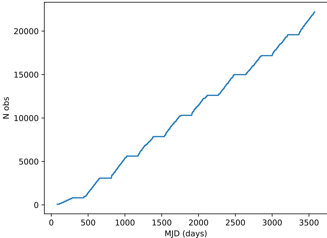
too_ignore_10_1v3.4_10yrs all bands: DD:XMM_LSS Cumulative NVisits
