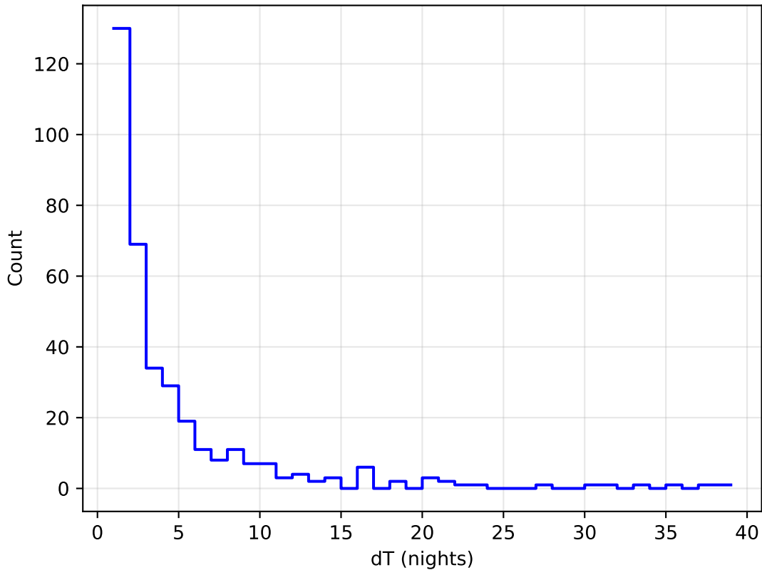
too_ignore_10_1v3.4_10yrs all bands: DD:WFD Delta Nights Histogram
