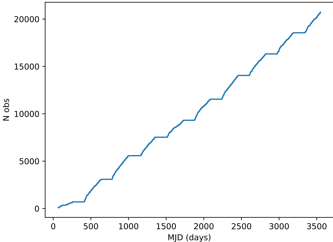
too_ignore_10_1v3.4_10yrs all bands: DD:ELAISS1 Cumulative NVisits
