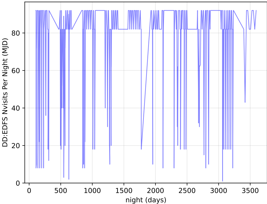
too_ignore_10_1v3.4_10yrs all bands: DD:EDFS Nvisits Per Night
