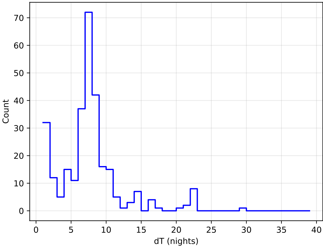
too_ignore_10_1v3.4_10yrs all bands: DD:EDFS Delta Nights Histogram
