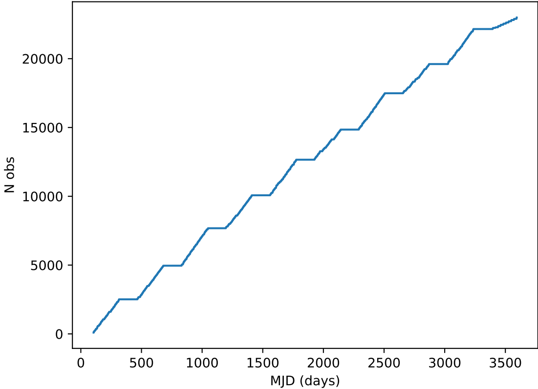
too_ignore_10_1v3.4_10yrs all bands: DD:EDFS Cumulative NVisits
