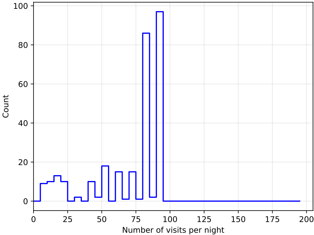
too_ignore_10_1v3.4_10yrs all bands: DD:ECDFS NVisitsPerNight
