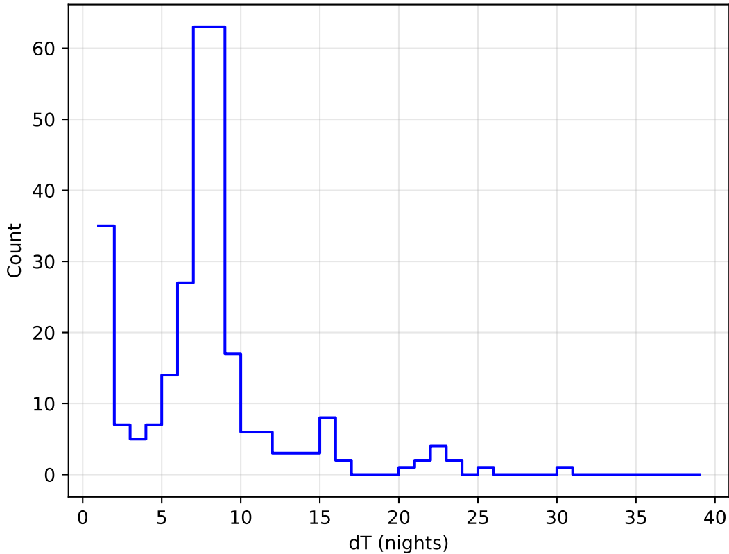
too_ignore_10_1v3.4_10yrs all bands: DD:ECDFS Delta Nights Histogram
