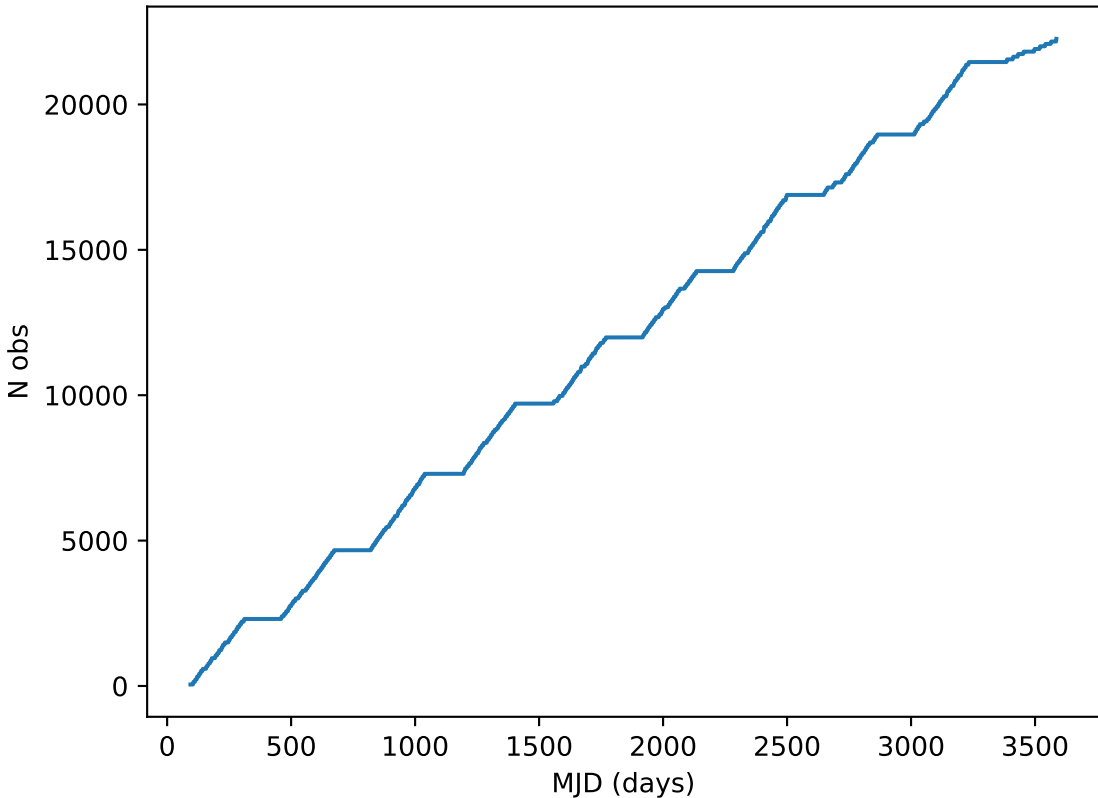
too_ignore_10_1v3.4_10yrs all bands: DD:ECDFS Cumulative NVisits
