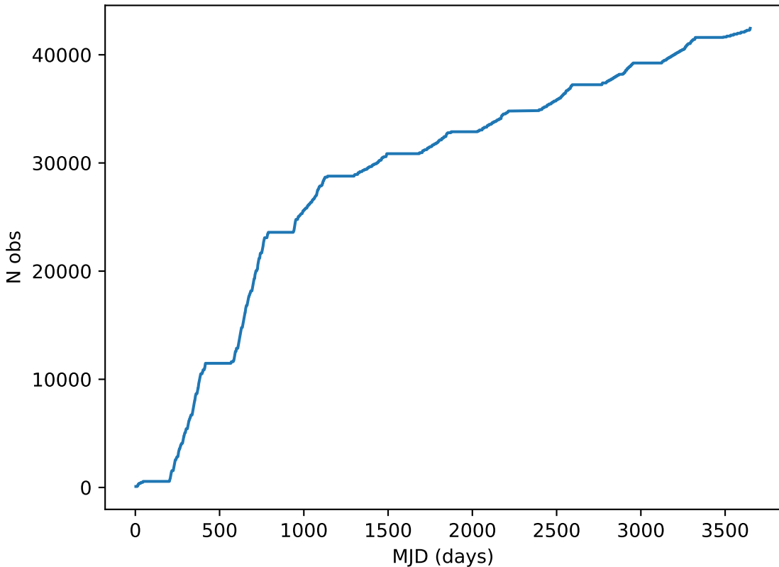
too_ignore_10_1v3.4_10yrs all bands: DD:COSMOS Cumulative NVisits
