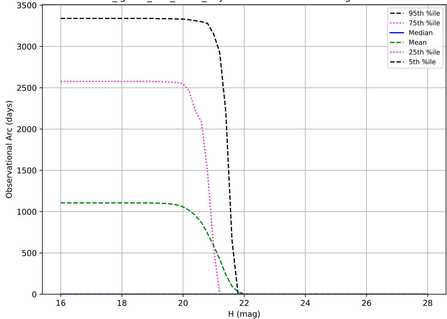
too_ignore_100_4v3.4_10yrs: Observational Arc Length Vatira
