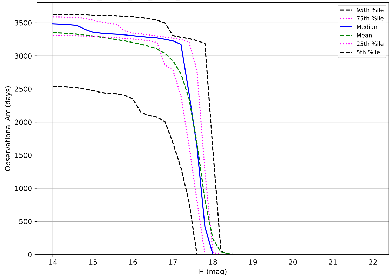
too_ignore_100_4v3.4_10yrs: Observational Arc Length Trojan
