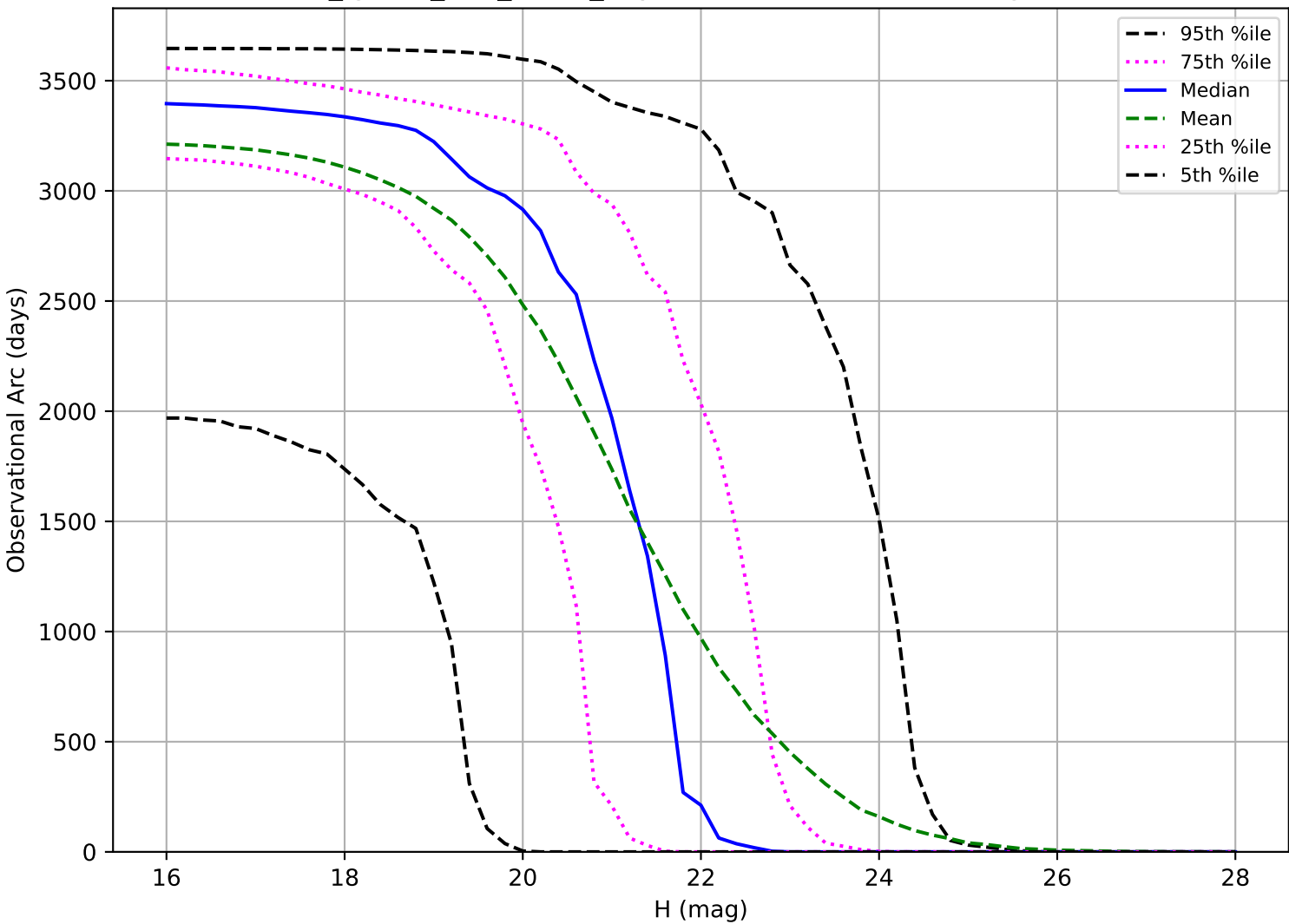
too_ignore_100_4v3.4_10yrs: Observational Arc Length PHA
