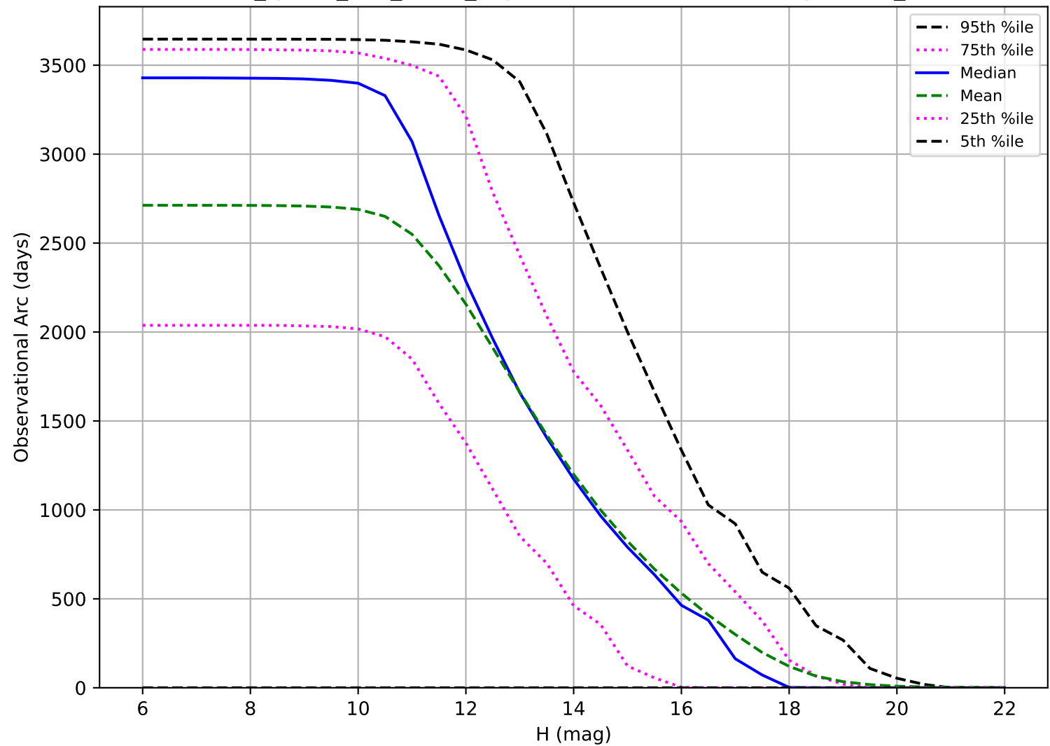
too_ignore_100_4v3.4_10yrs: Observational Arc Length OCC_r5
