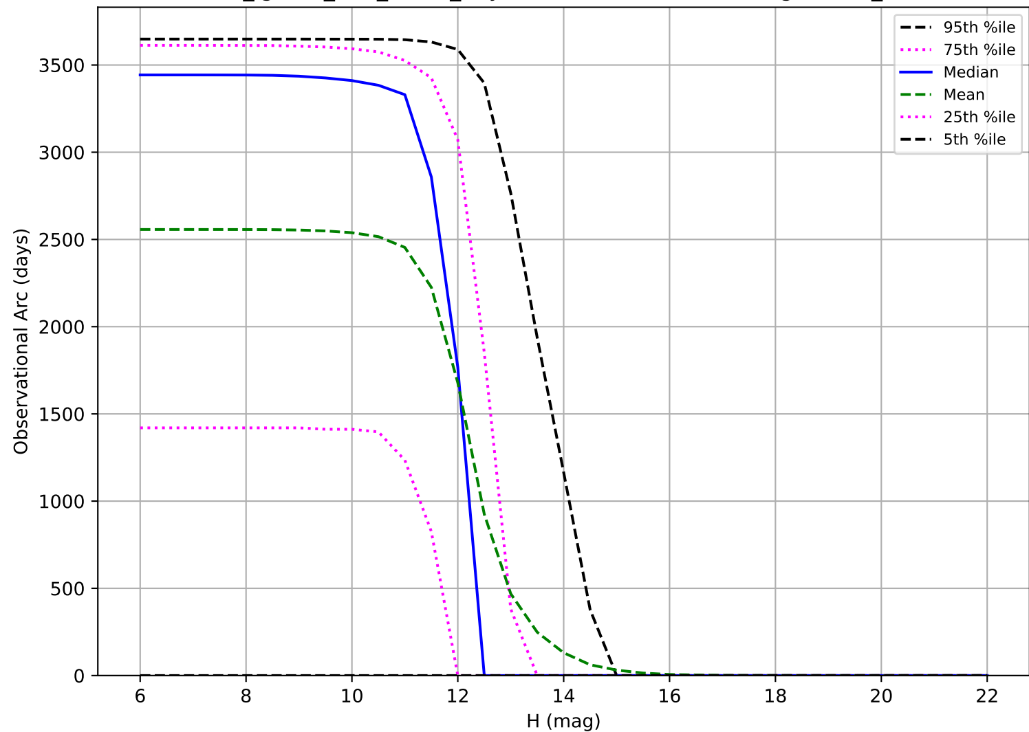
too_ignore_100_4v3.4_10yrs: Observational Arc Length OCC_r20
