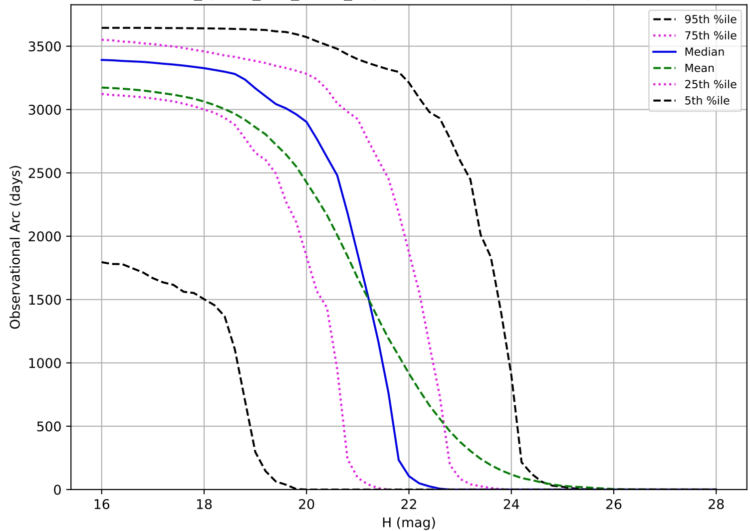
too_ignore_100_4v3.4_10yrs: Observational Arc Length NEO
