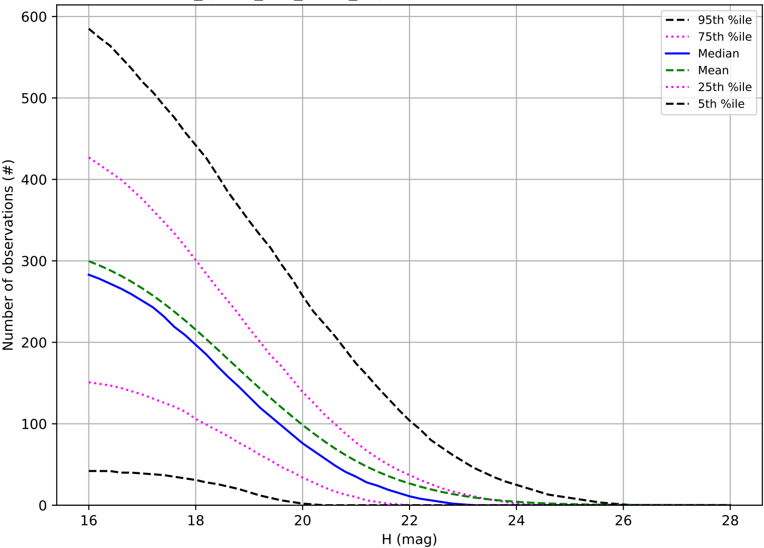
too_ignore_100_4v3.4_10yrs: Number of observations PHA
