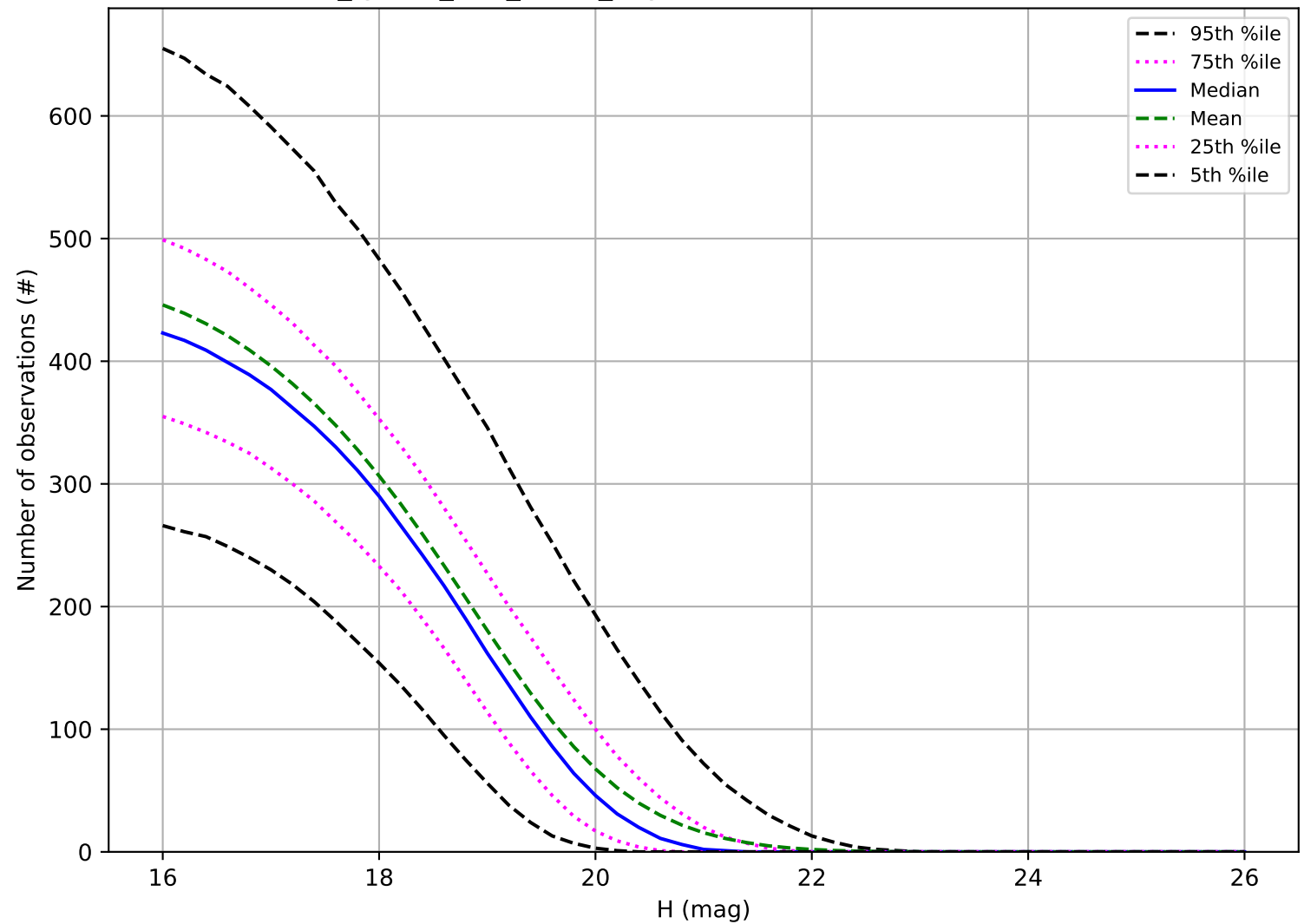
too_ignore_100_4v3.4_10yrs: Number of observations MBA
