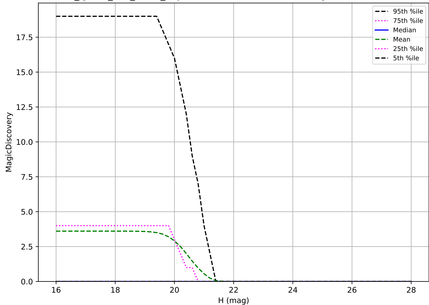
too_ignore_100_4v3.4_10yrs: Vatira 6 detections in 60 nights detection loss
