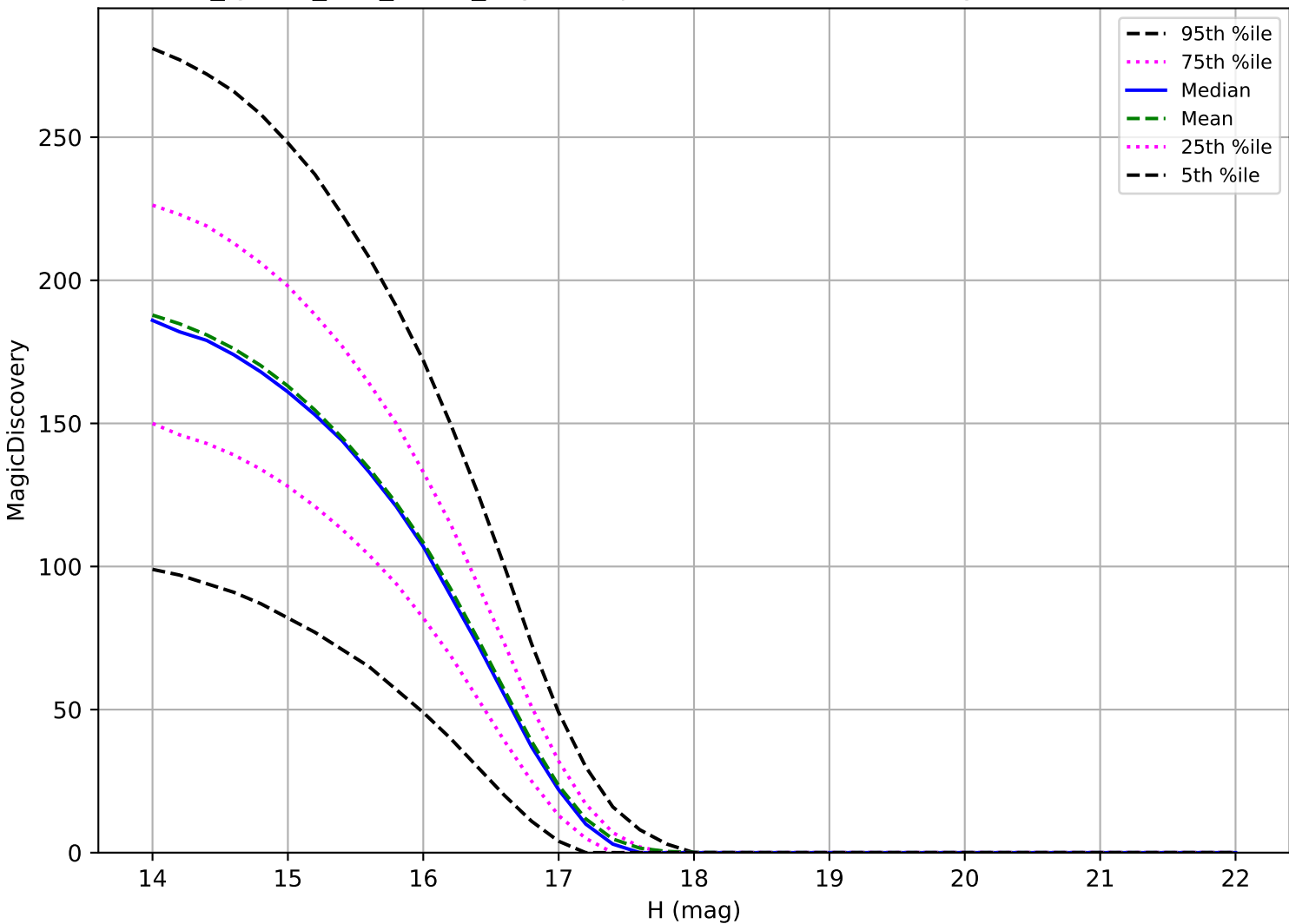
too_ignore_100_4v3.4_10yrs: Trojan 6 detections in 60 nights detection loss
