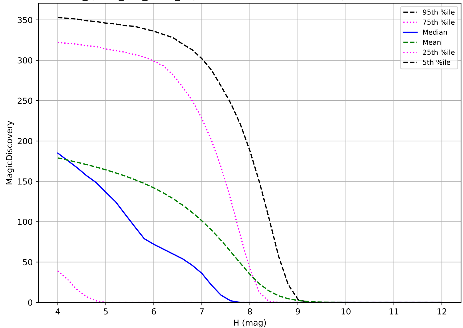
too_ignore_100_4v3.4_10yrs: TNO 6 detections in 60 nights detection loss
