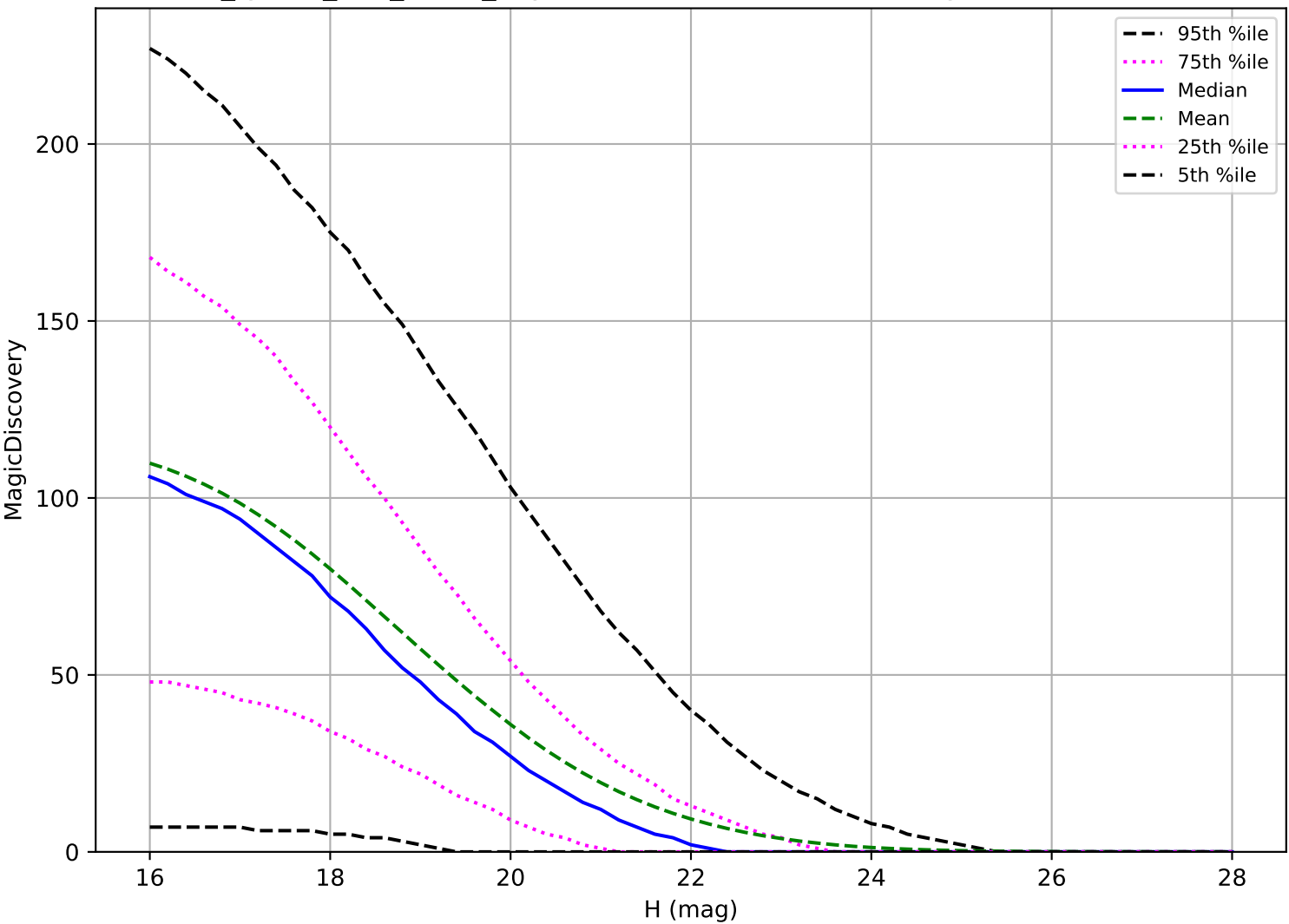
too_ignore_100_4v3.4_10yrs: PHA 6 detections in 60 nights detection loss
