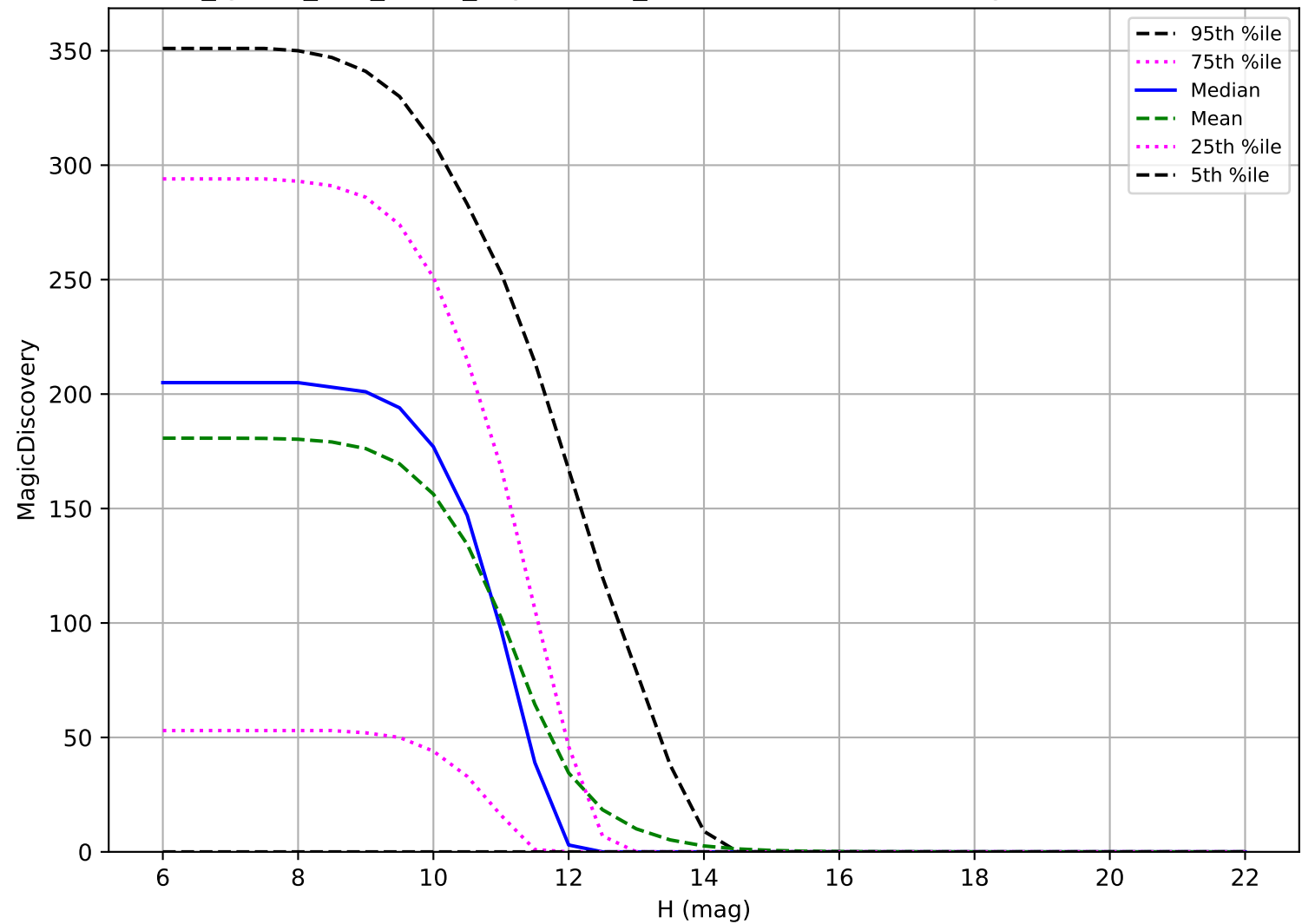
too_ignore_100_4v3.4_10yrs: OCC_r20 6 detections in 60 nights detection loss
