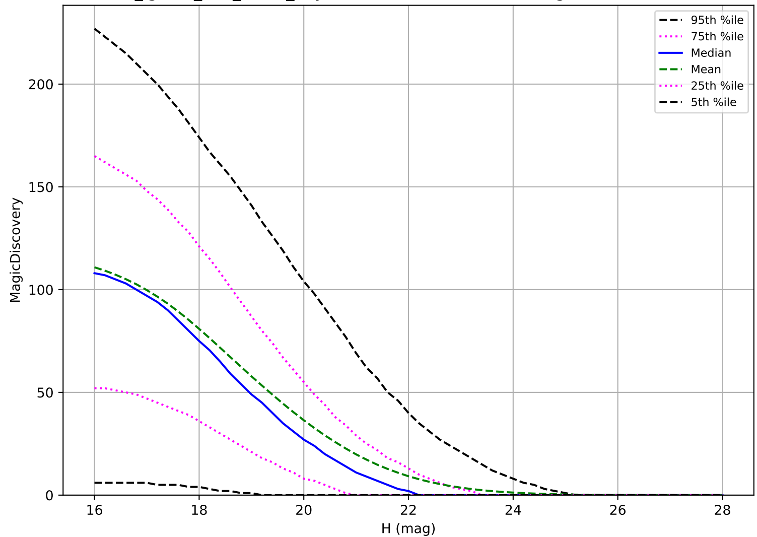
too_ignore_100_4v3.4_10yrs: NEO 6 detections in 60 nights detection loss
