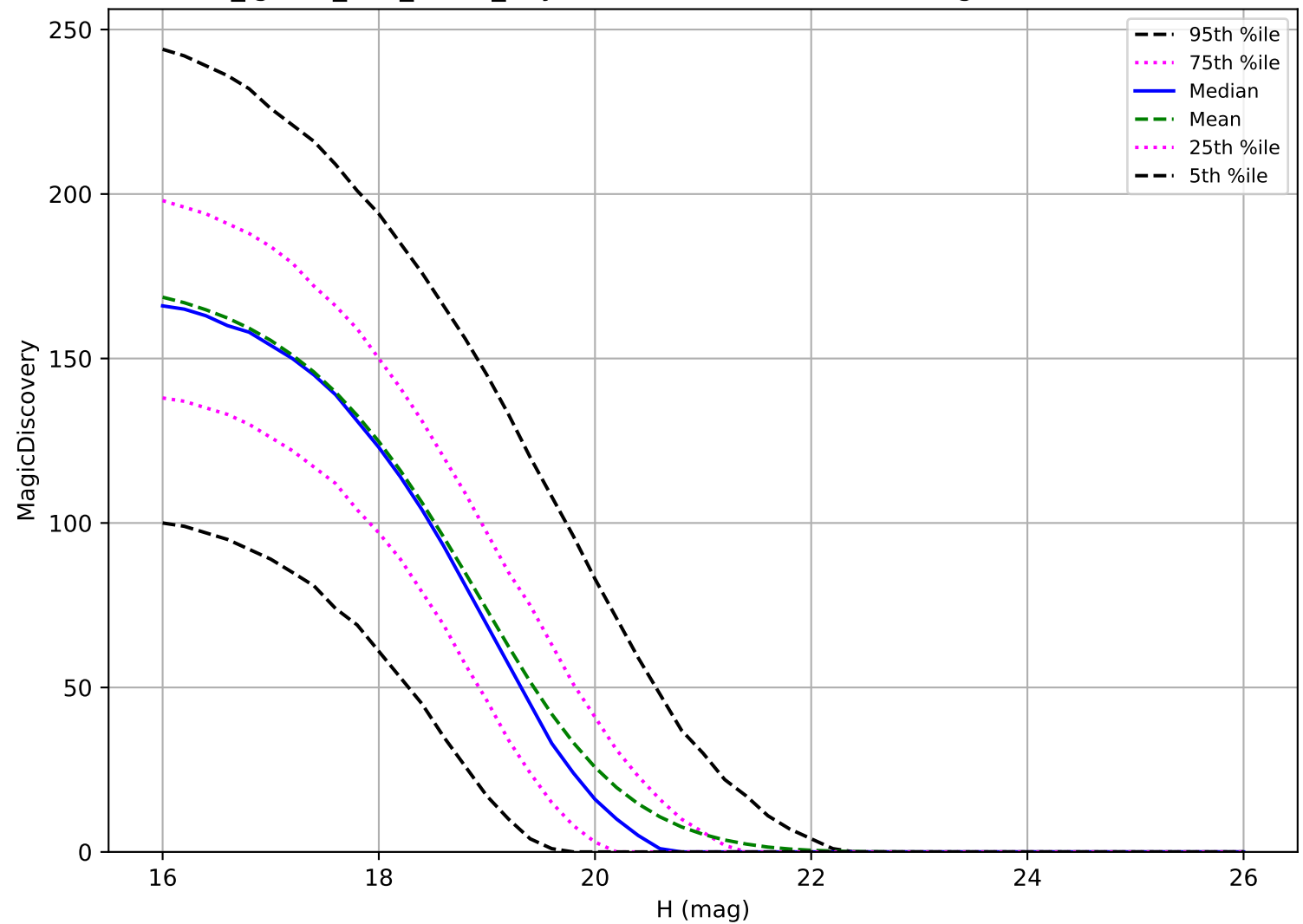
too_ignore_100_4v3.4_10yrs: MBA 6 detections in 60 nights detection loss
