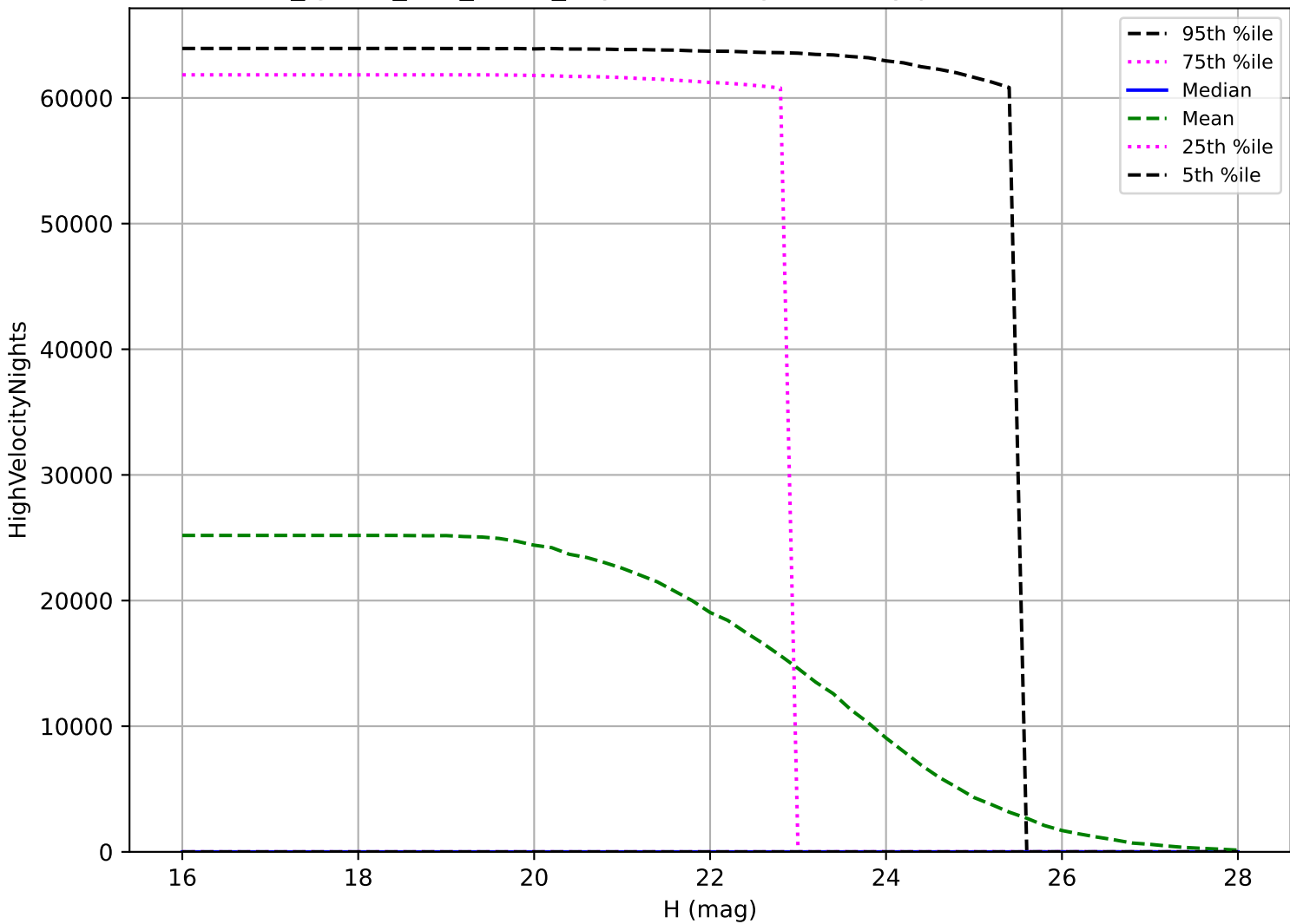
too_ignore_100_4v3.4_10yrs: PHA High velocity pair detection loss
