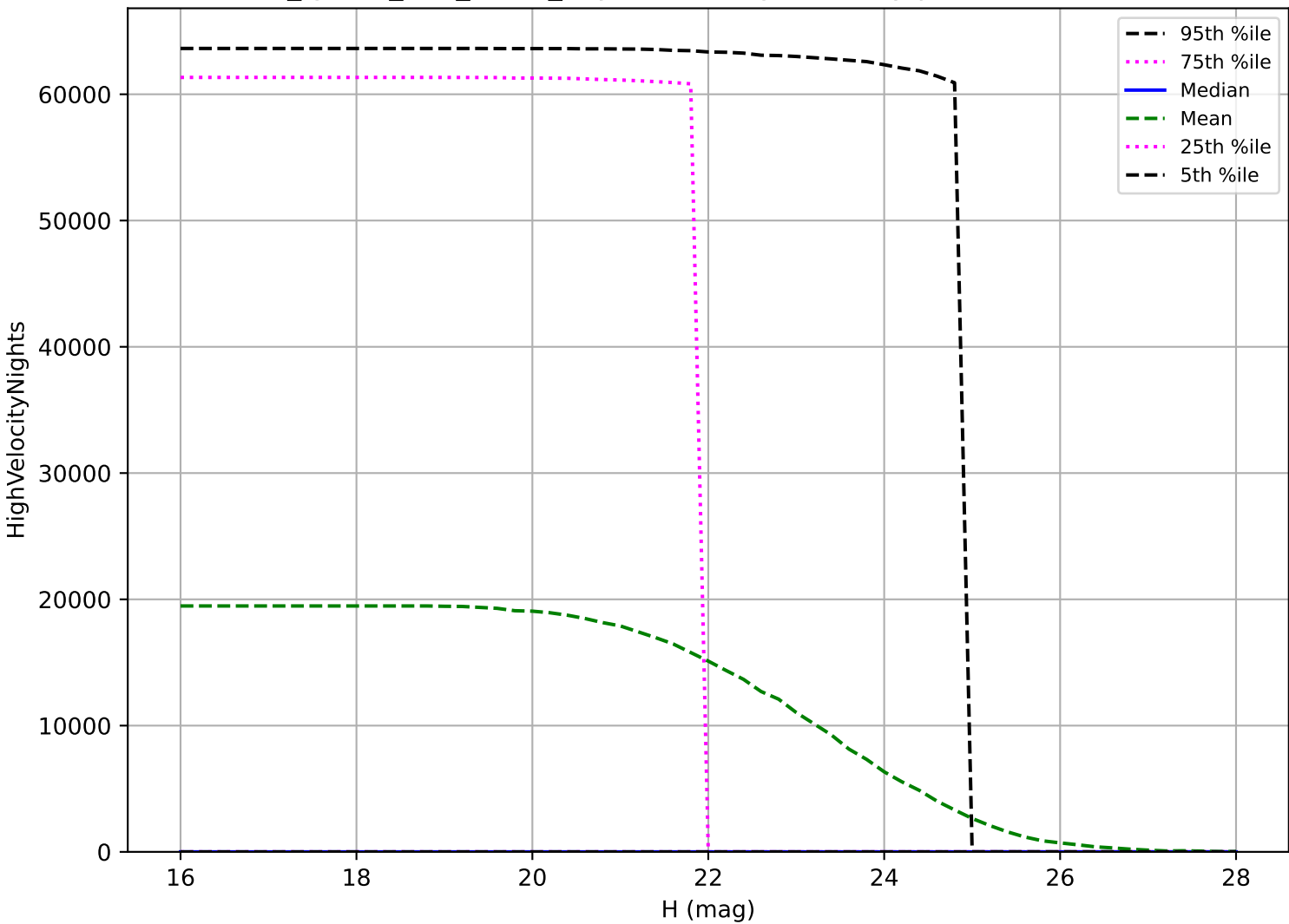
too_ignore_100_4v3.4_10yrs: NEO High velocity pair detection loss
