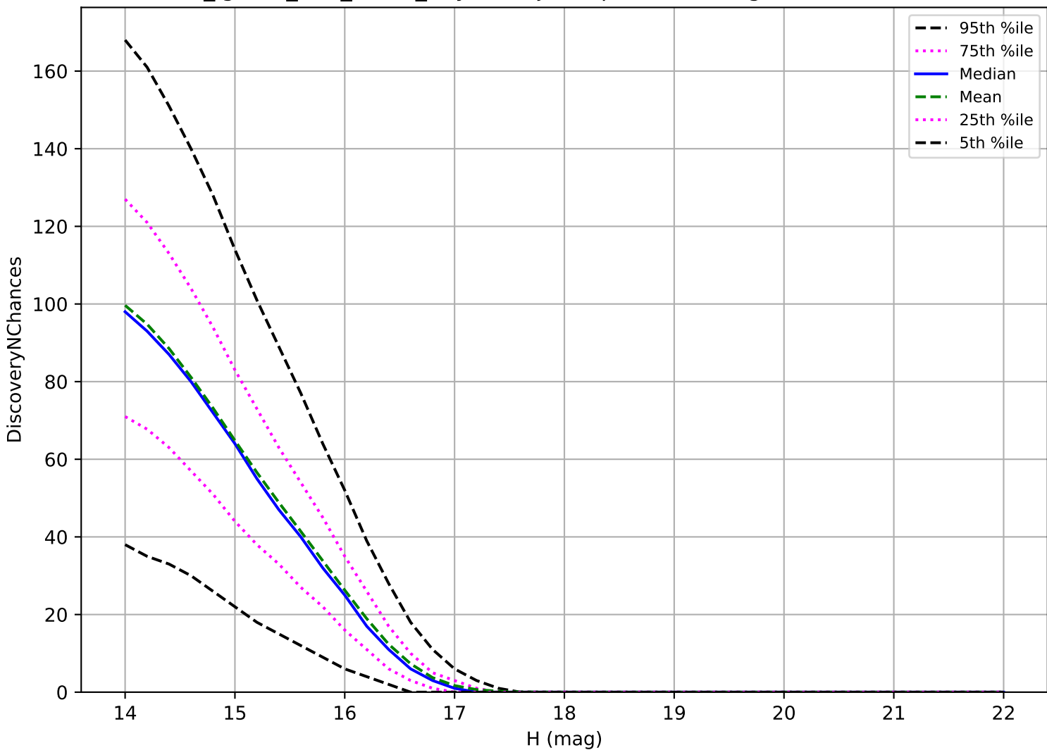
too_ignore_100_4v3.4_10yrs: Trojan 3 pairs in 15 nights detection loss
