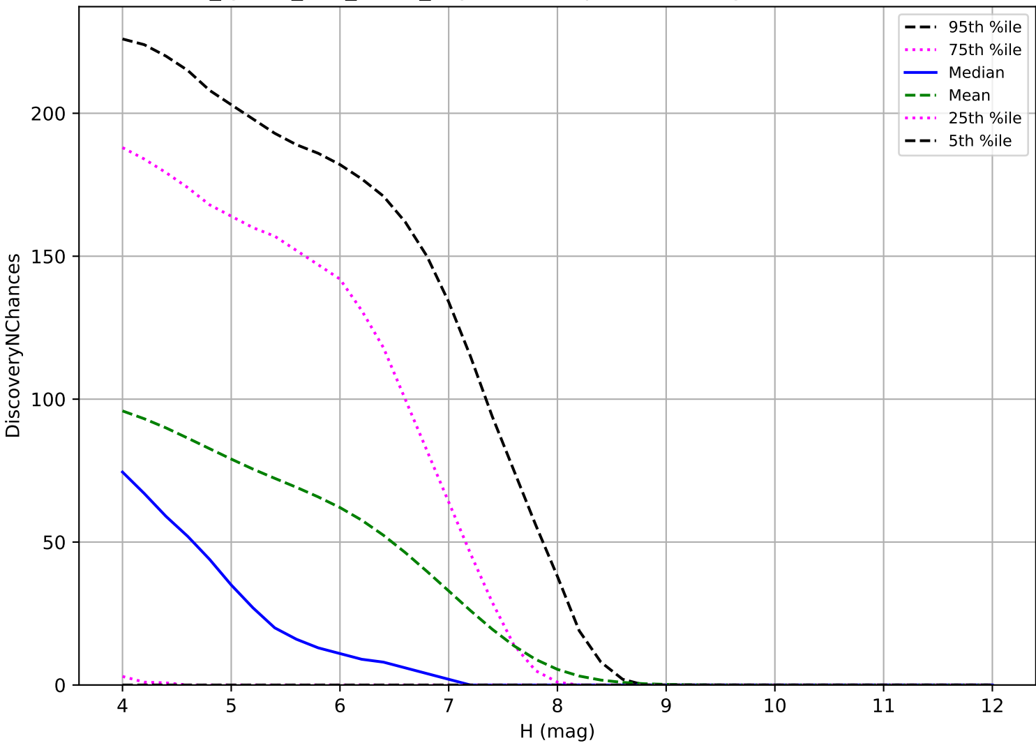
too_ignore_100_4v3.4_10yrs: TNO 3 pairs in 15 nights detection loss
