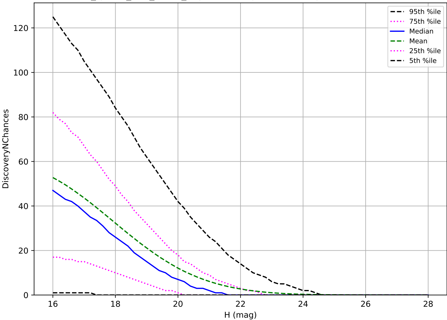
too_ignore_100_4v3.4_10yrs: PHA 3 pairs in 15 nights detection loss
