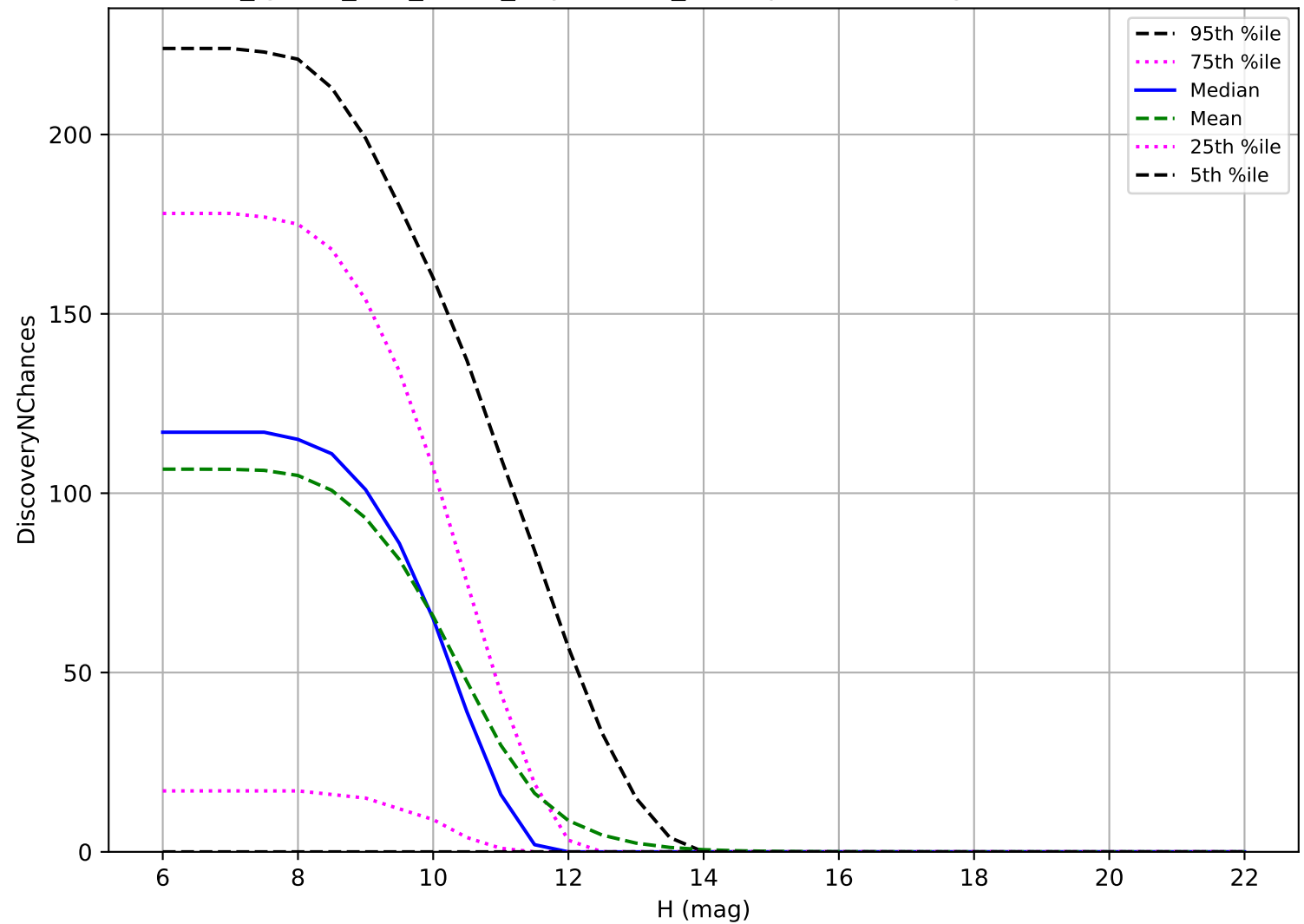
too_ignore_100_4v3.4_10yrs: OCC_r20 3 pairs in 15 nights detection loss
