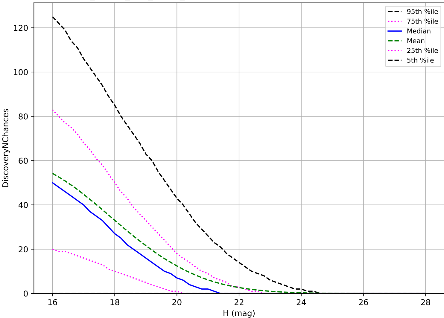
too_ignore_100_4v3.4_10yrs: NEO 3 pairs in 15 nights detection loss
