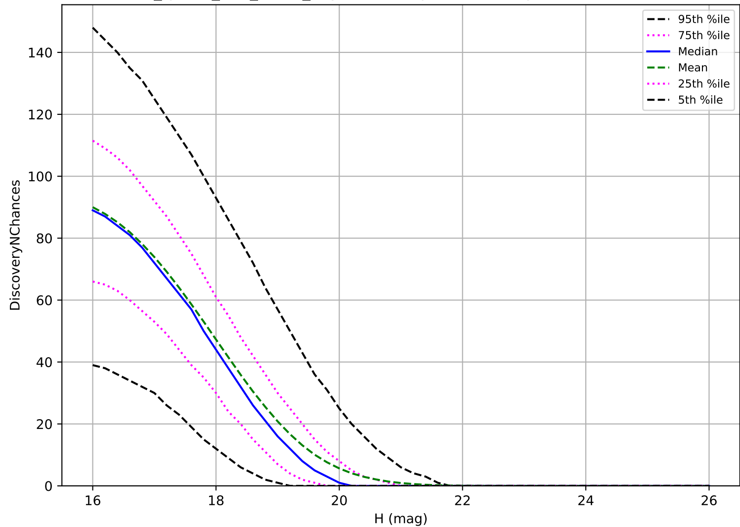
too_ignore_100_4v3.4_10yrs: MBA 3 pairs in 15 nights detection loss
