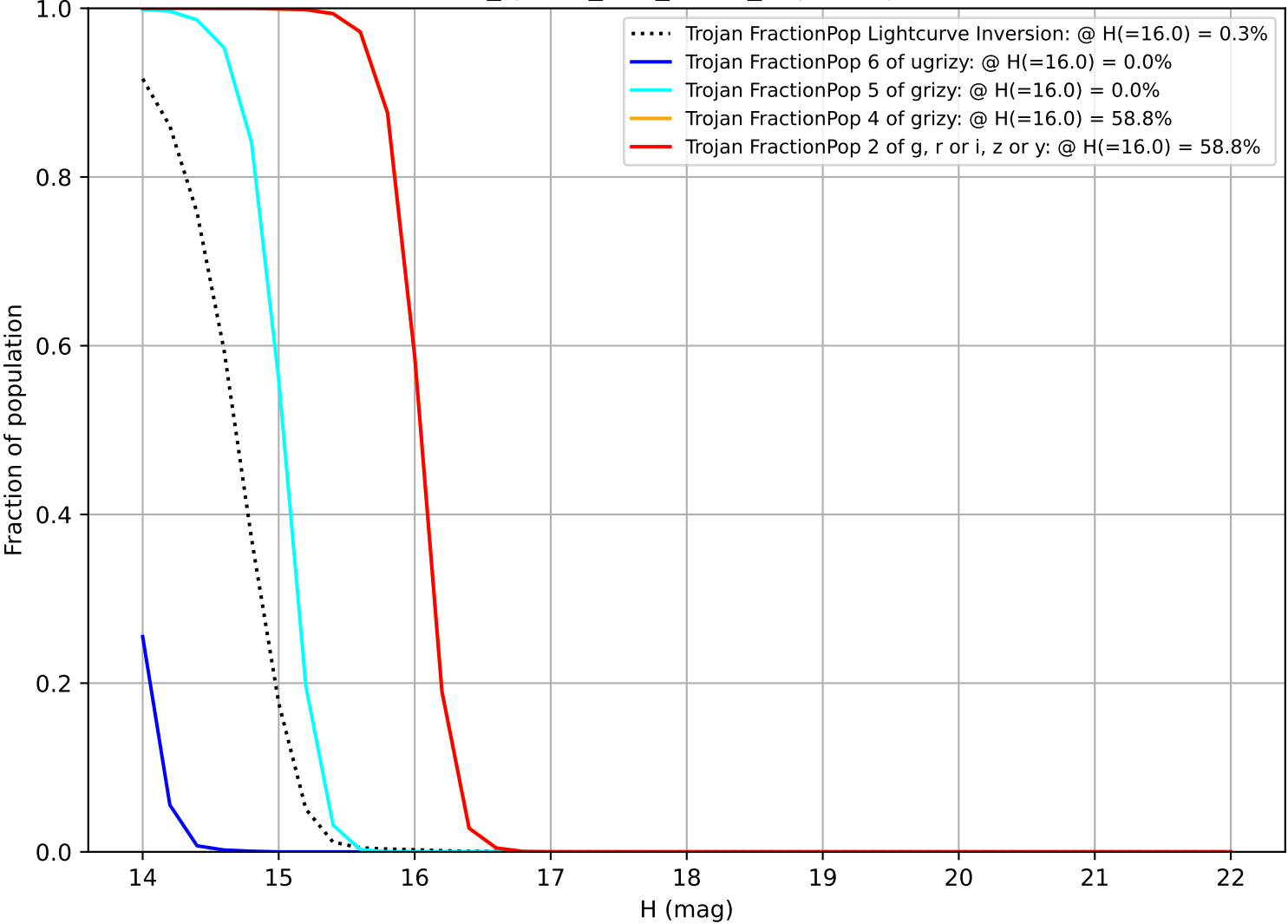
too_ignore_100_4v3.4_10yrs Trojan
