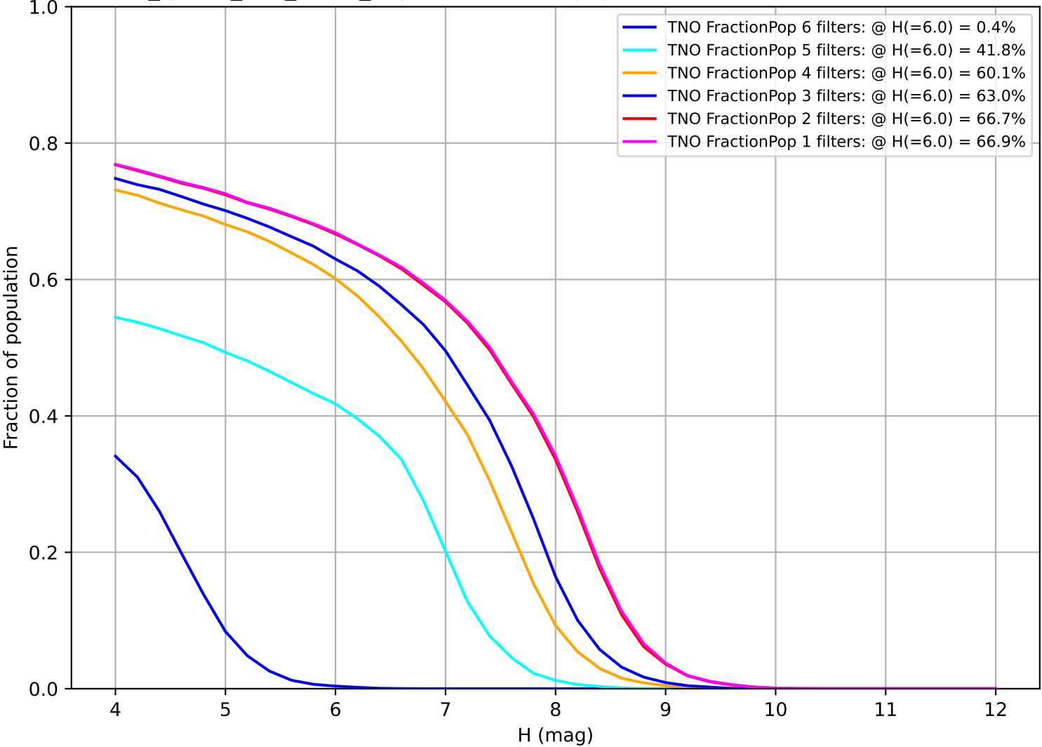
too_ignore_100_4v3.4_10yrs: Fraction of population with colors in X filters TNO
