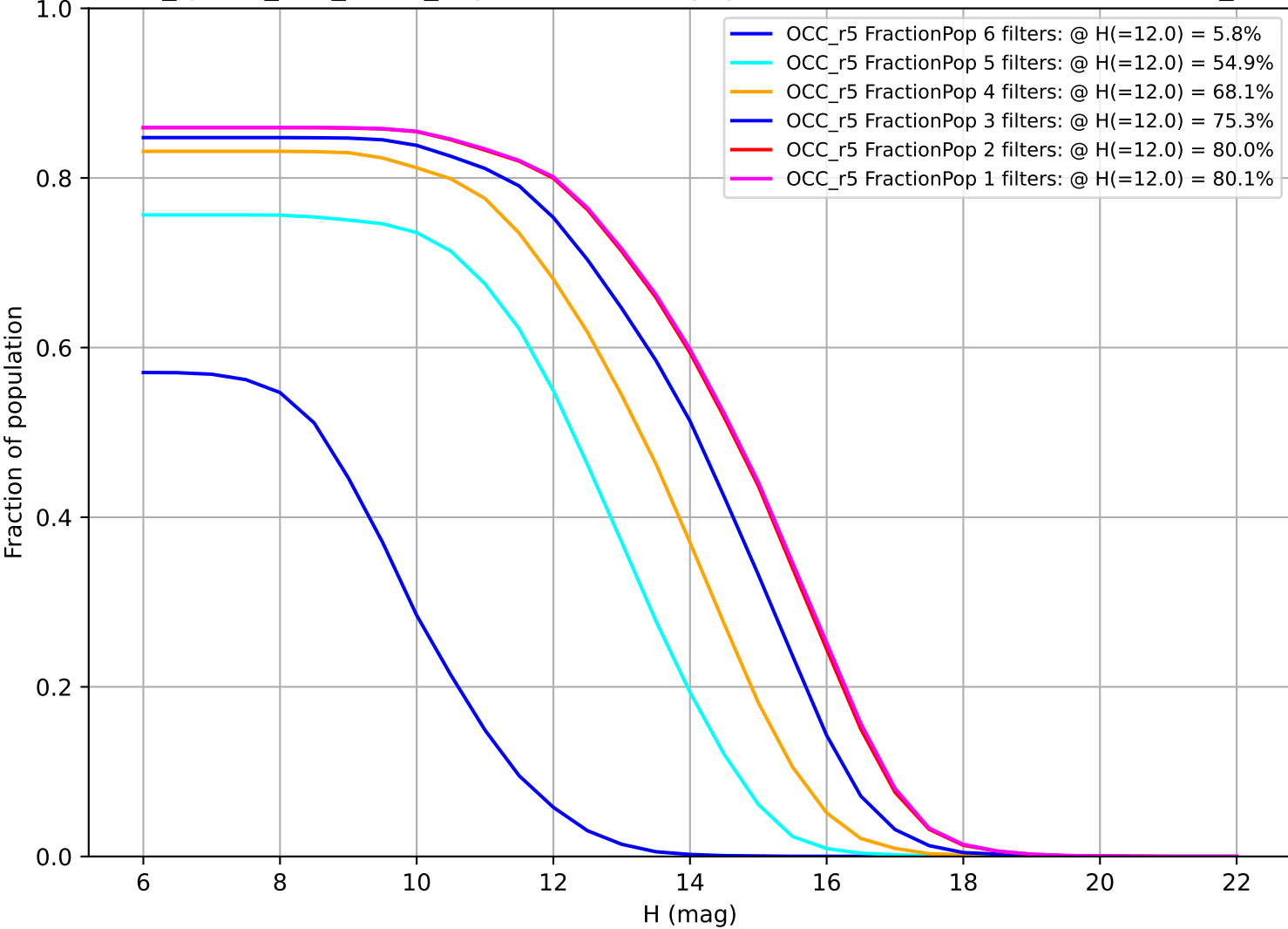
too_ignore_100_4v3.4_10yrs: Fraction of population with colors in X filters OCC_r5
